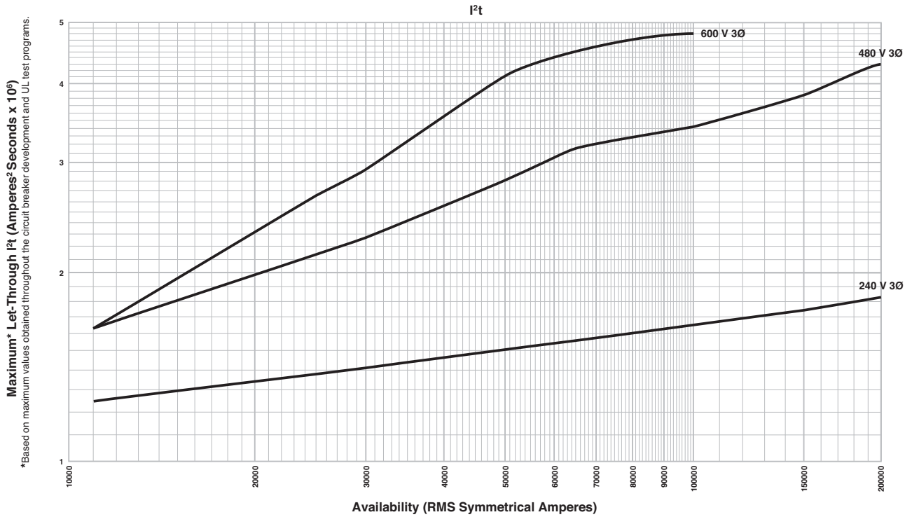
Figure 113: L-Frame Circuit Breaker Reflex Tripping
