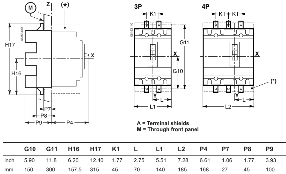
Figure 35: PowerPact L-Frame Plug-In Circuit Breaker (On Base)
