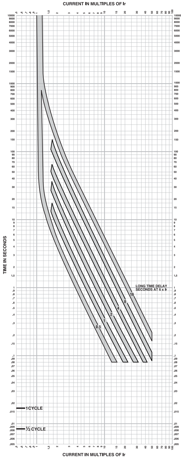
Figure 91: Micrologic 5.2A/5.2E/6.2A/6.2E Electronic Trip Unit Long Time Trip Curve
