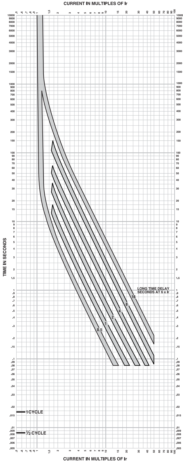
Figure 106: Micrologic 5.3A/5.3E/6.3A/6.3E Electronic Trip Unit Long Time Trip Curve
