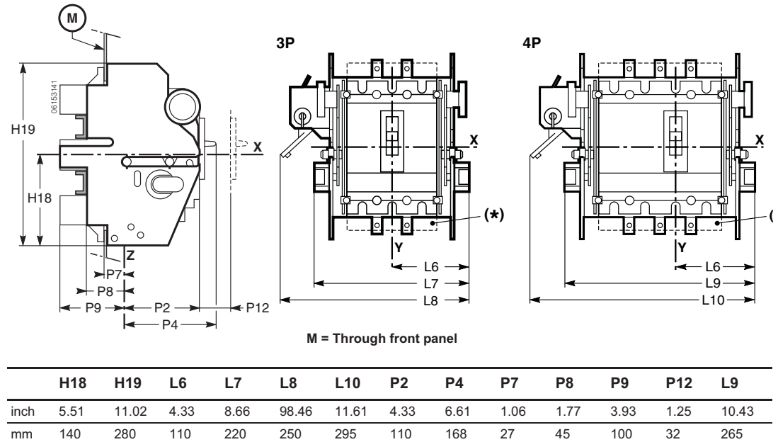
Figure 36: PowerPact L-Frame Drawout Circuit Breaker (on Cradle)
