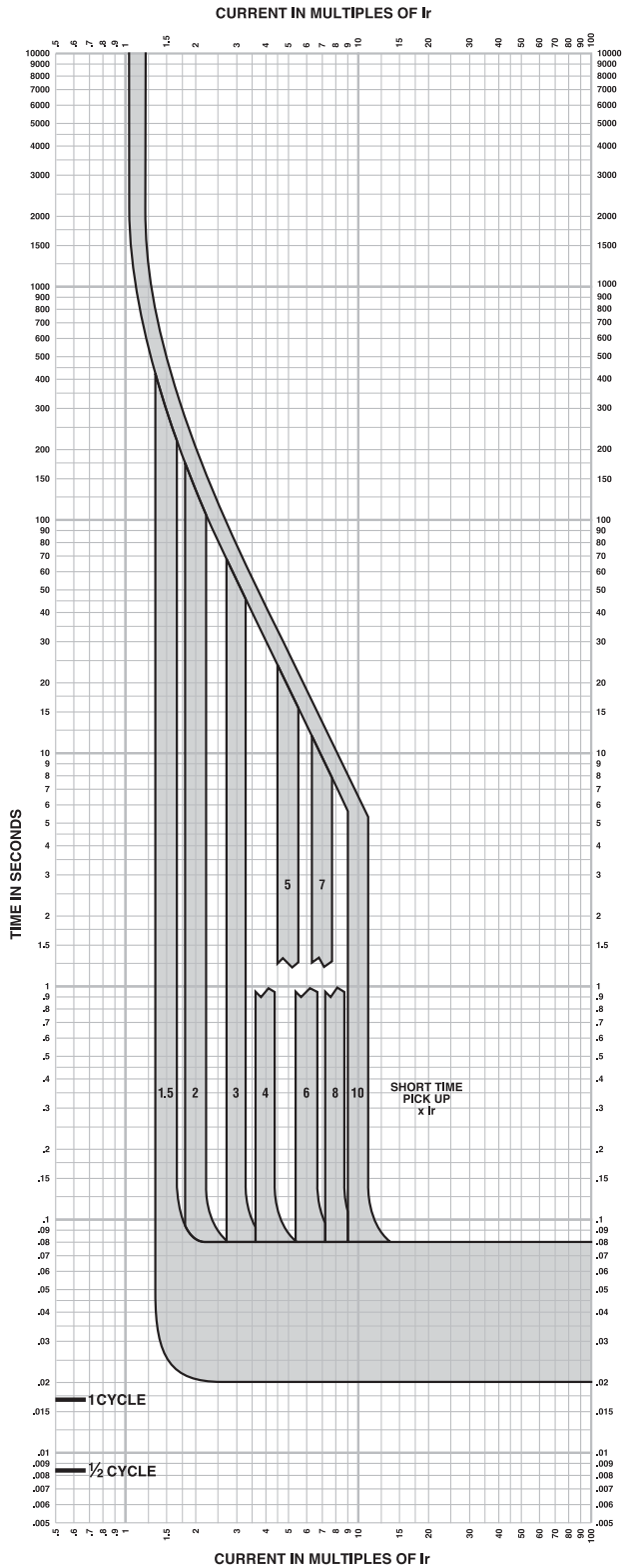
Figure 89: Micrologic 3.2S Electronic Trip Unit Long Time / Short Time Trip Curve
