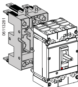
Plug-In Mounting
